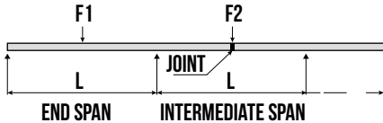
H 100 R5 WIRE MESH CABLE TRAY SWL PER 1.5M SPAN
