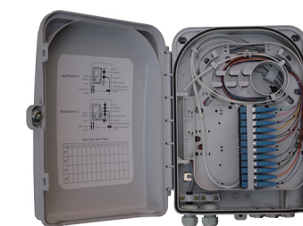
Optical Termination Box
