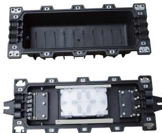
Optical Cable Splice Closure
