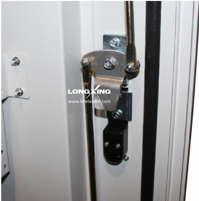
Lock & anti theft U-bar protection
