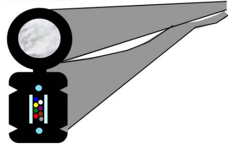
SSW Aerial Cable
