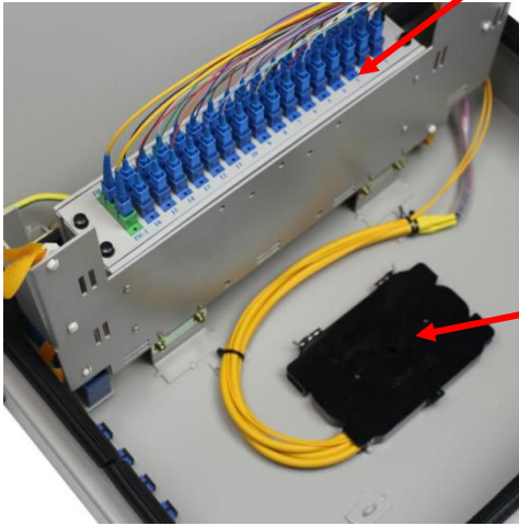
Micro splitter
